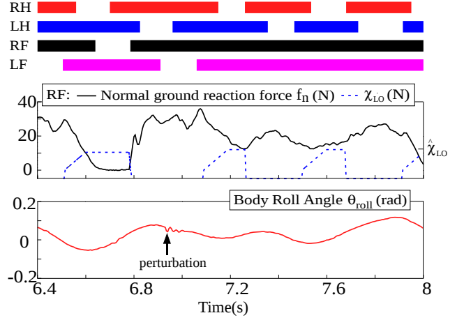
Fig. 1 Results of an experiment against the lateral perturbation without ACM exc and ACM w . Alternation of leg loading between contralateral legs was prevented, and leg loading of RF was kept high. Since max value of \chi_{LO} was constant, the stance-to-swing phase transition of RF was not initiated. Consequently Kotetsu fell down to the right side.
