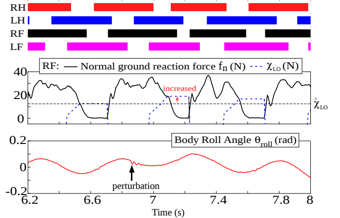
Fig. 2 Results of an experiment against the lateral perturbations with ACM exc and ACM w . Although leg loading of RF was kept high, the stance-to-swing phase transition of RF was initiated because max value of \chi_{LO} was increased by ACM exc . Consequently the gait was stabilized and Kotetsu kept walking.
