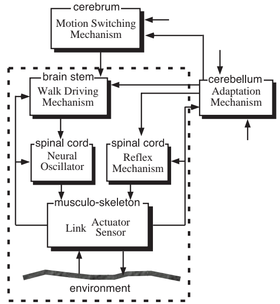
Figure 2: Primitive control mechanism of legged locomotion in animals.
