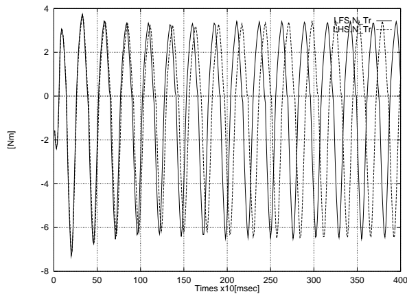
Figure 14: Results of the experiment involving the gait transition from standing to bouncing via hopping: LFS.N.Tr and LHS.N.Tr are, respectively, the joint torques of the hip joints of the left foreleg and left hindleg.
