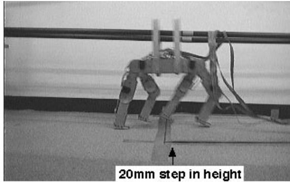
Figure 9: Photo of the quadruped walking up a step.
