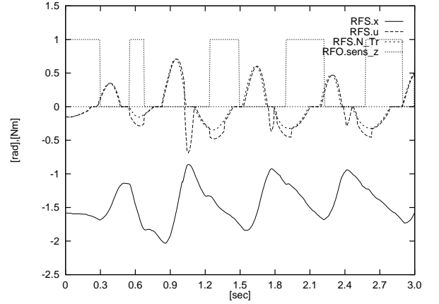
Figure 7: Results of the experiment involving walking on flat terrain using the stretch reflex: RFS.x and RFS.N\_Tr are, respectively, the angle and the output torque of the N.O. of the hip joint of the right foreleg. RFO.sens\_z is the vertical contact sensor output of the right foreleg. RFS.u is the joint torque, which is the sum of RFS.N\_Tr and the output torque of the reflex mechanism.
