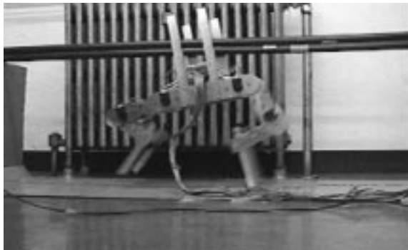
Figure 15: Photos of the quadruped running in a bounce gait.
