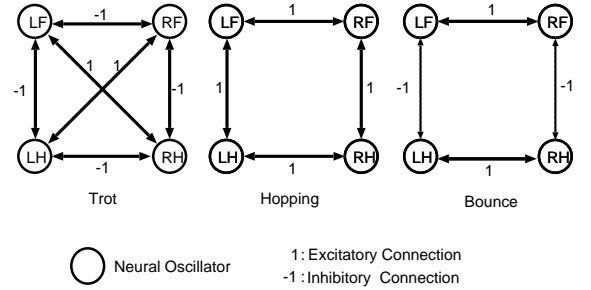
Figure 4: Neural oscillator networks for walking (a trot gait) and running (hopping and bounce gaits). An excitatory connection makes the phase difference between legs zero. An inhibitory connection makes the phase difference 180 degrees. LF, LH, RF and RH stand for left foreleg, left hindleg, right foreleg and right hindleg, respectively.
